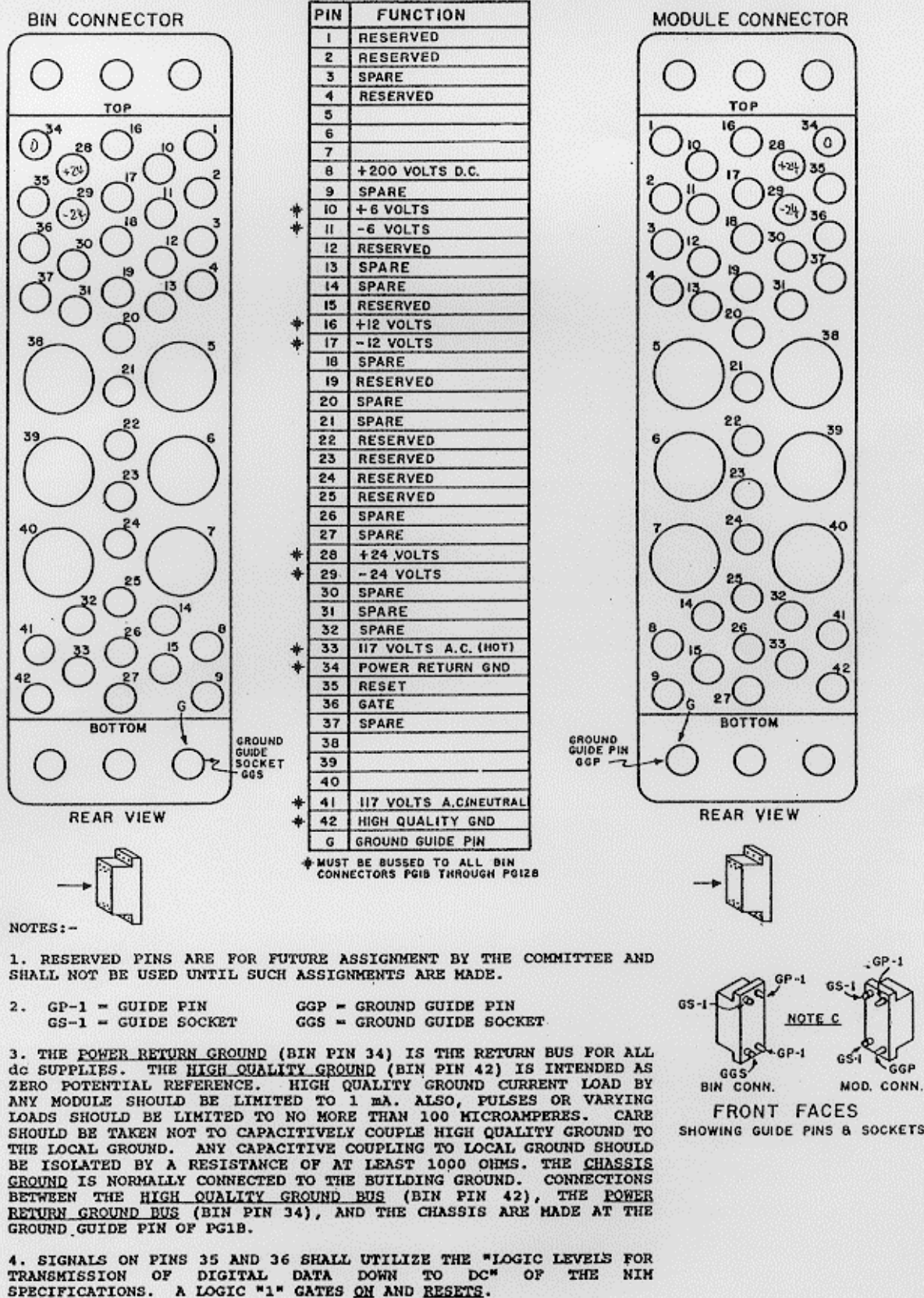
Figure 6. Bin and Module Connector Pin Assignments
